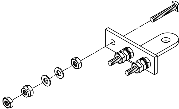
BATTERY TERMINAL 225481-000
