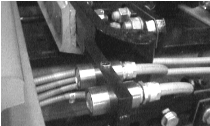
Sensor configuration for switch point detection. Both normal and reverse points are detected. Other applications include Bridge Signal and Dragging Equipment Detection
